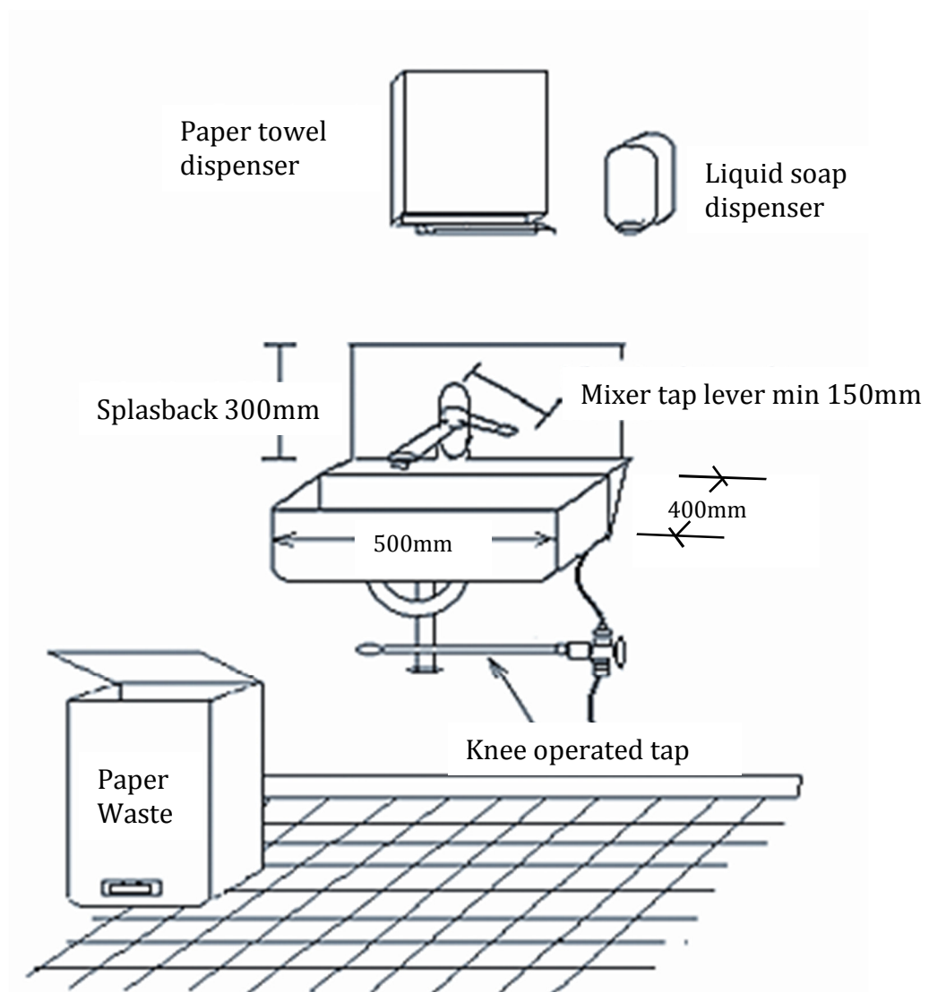
Figure 7: Typical hand washing facilities
