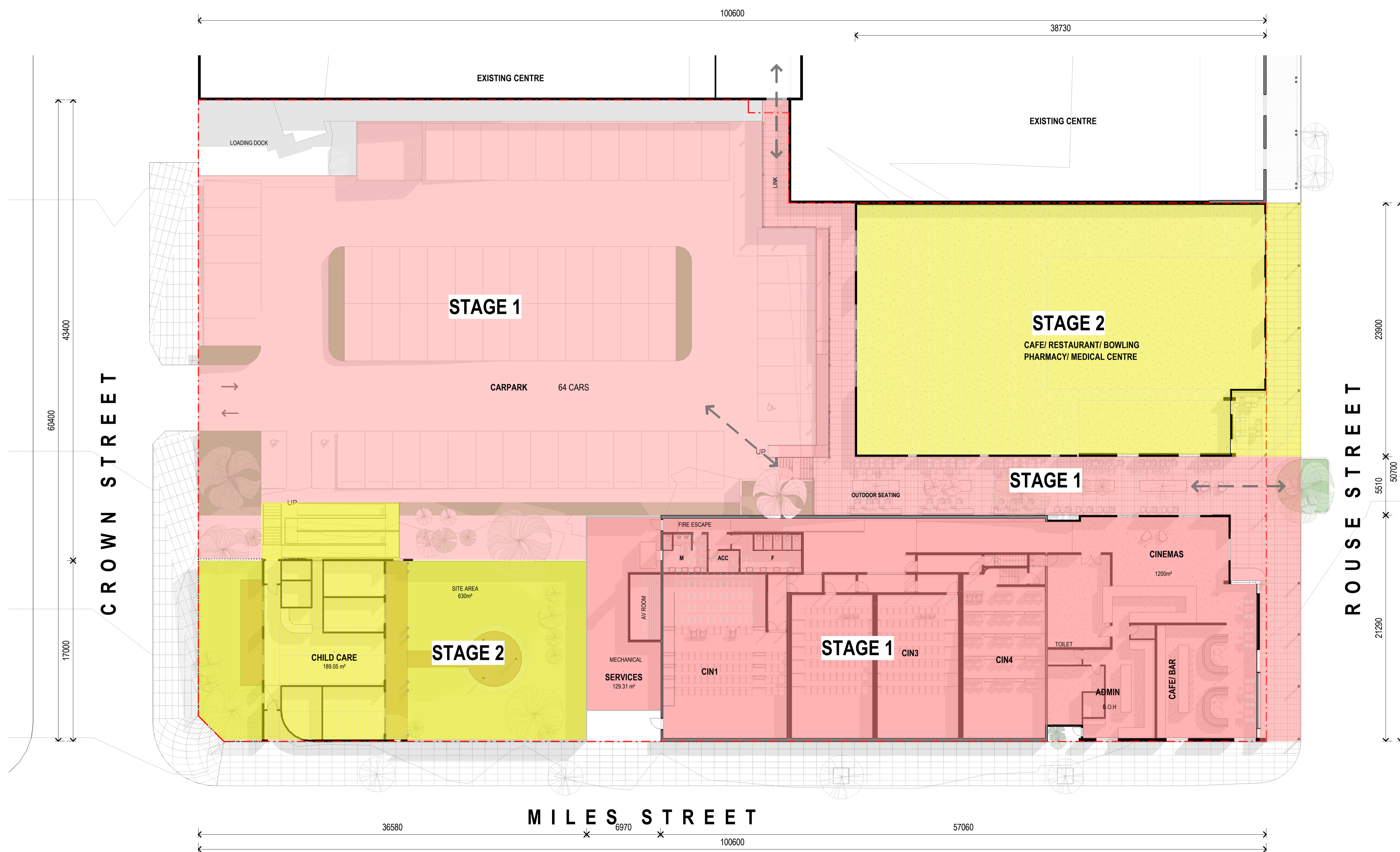
STAGING PLAN SCALE 1:200
