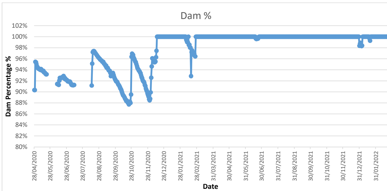
Graph 2 New Data logger Dam % Graph
