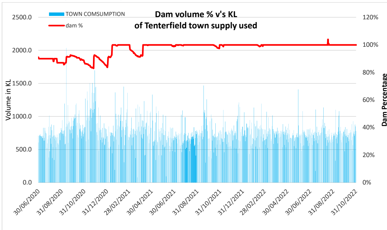
Graph 1 Dam % Levels and Consumption
