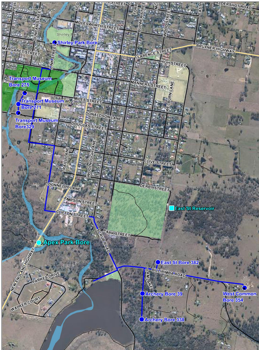
Figure 6-3 Tenterfield Bore Network
