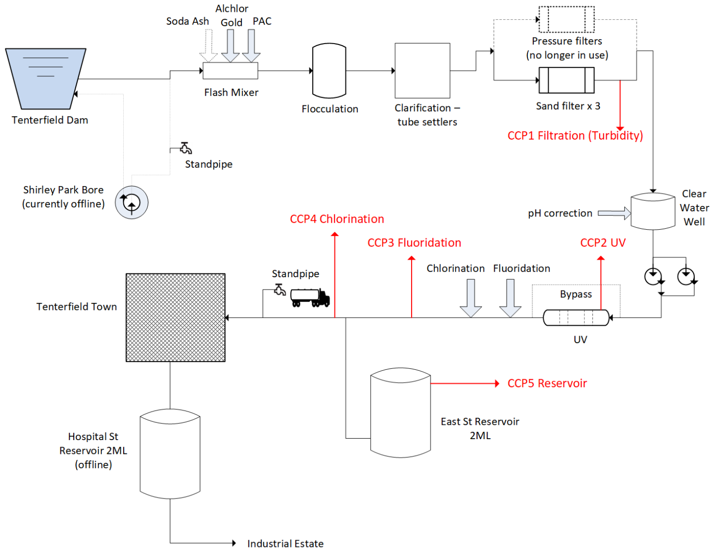
Figure 6-4 Tenterfield Water Supply Schematic (Viridis, 2018)
