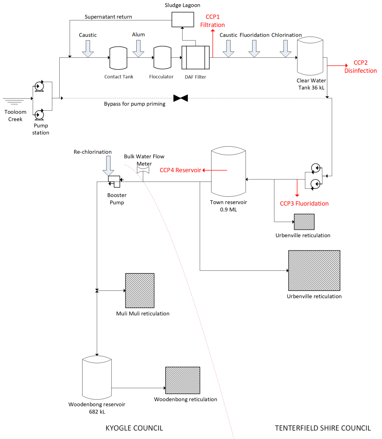
Figure 7-2 Urbenville Water Supply Schematic (Viridis, 2018)
